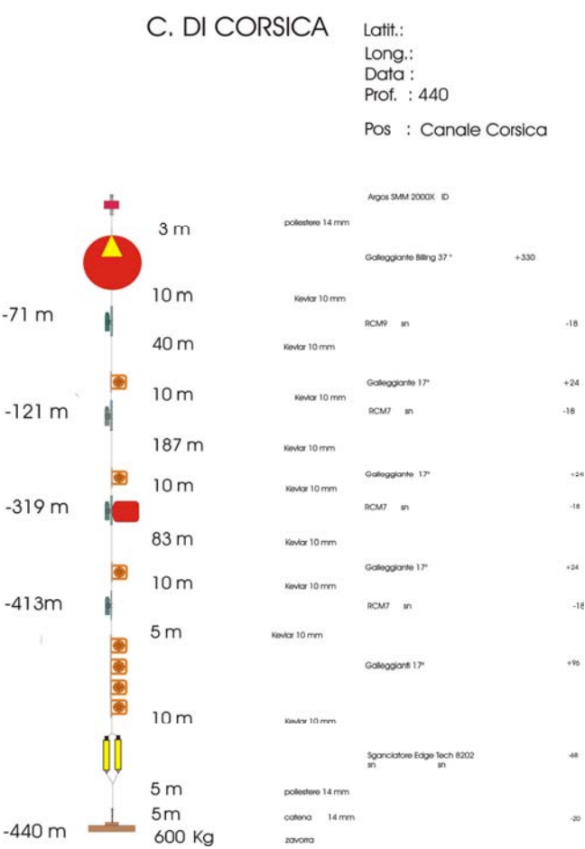
Figure 12 Scheme of the C. Channel mooring, in position 43°02.00' N and 009°415.00' E
